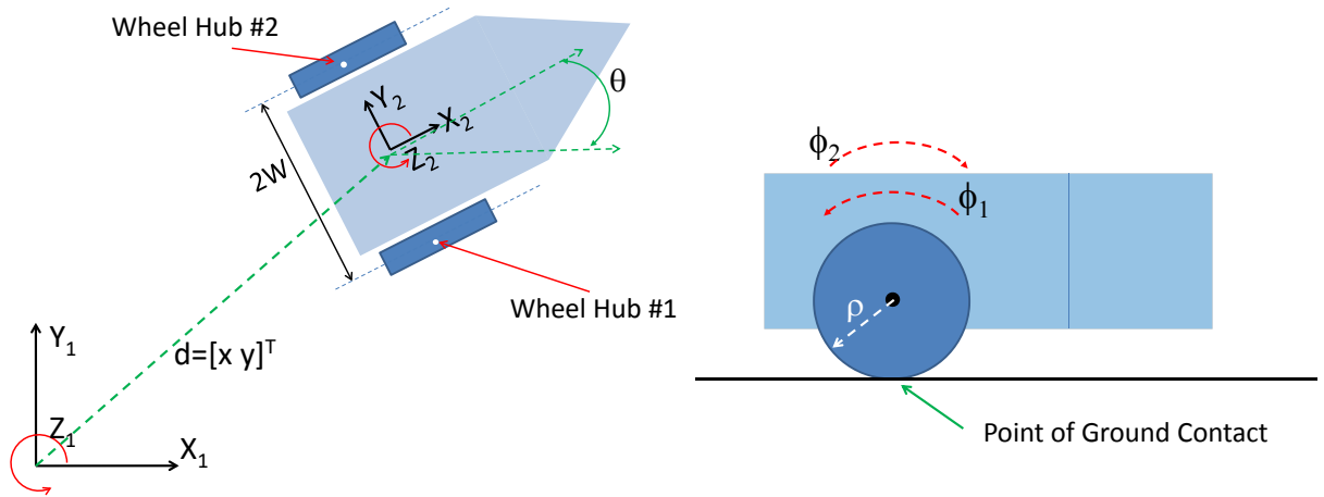
Figure 1: Schematic diagram of an idealized differential drive vehicle. The pointed end of the body is meant to convey the forward direction of the robot. Left: top view of the vehicle. Right: Side view of the vehicle.
